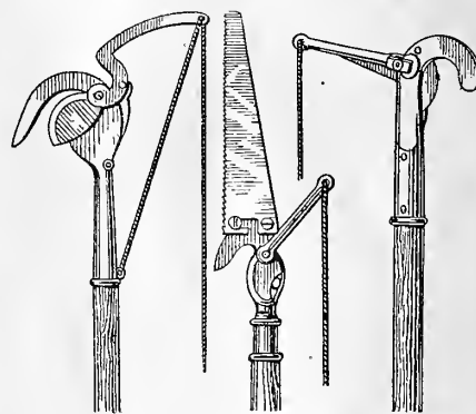
Disston's Little Giant
